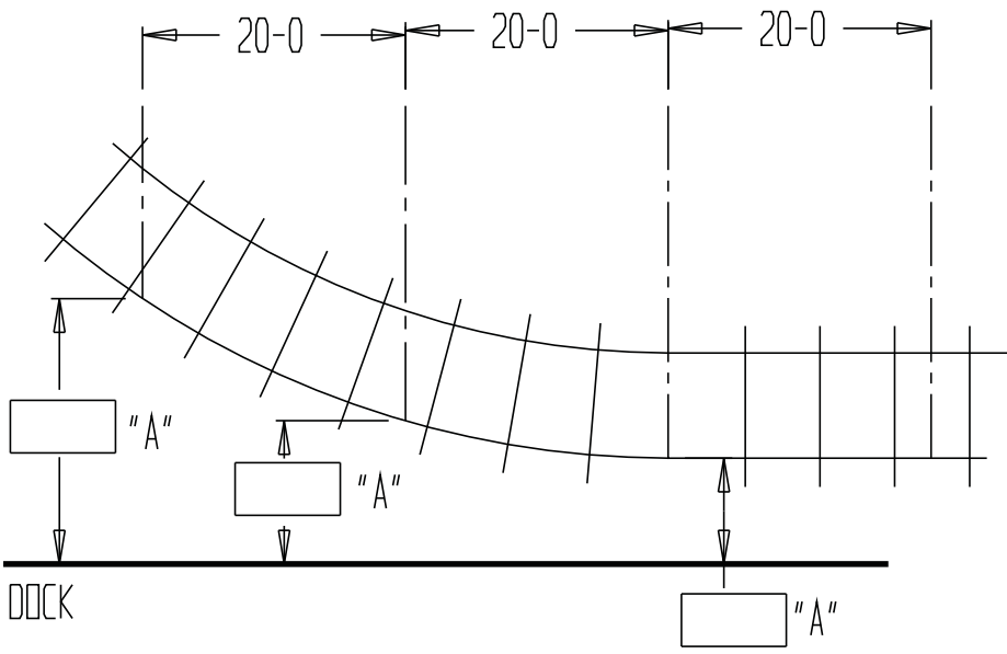
CURVED OR SKEWED TRACK WITH STRAIGHT DOCK
