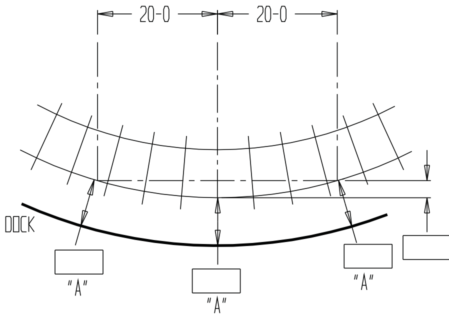
CURVED TRACK WITH CURVED DOCK
