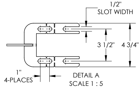
DETAIL A SCALE 1 : 5 DIMENSION TOLERANCE ± 1/4"
