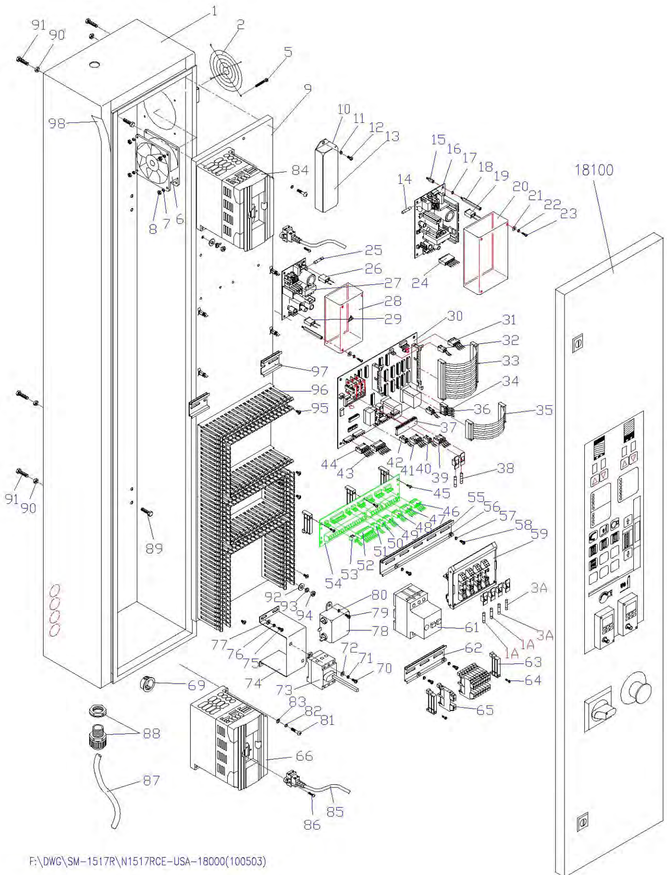
12-4-1 Fig-18000 Control Box Diagram
