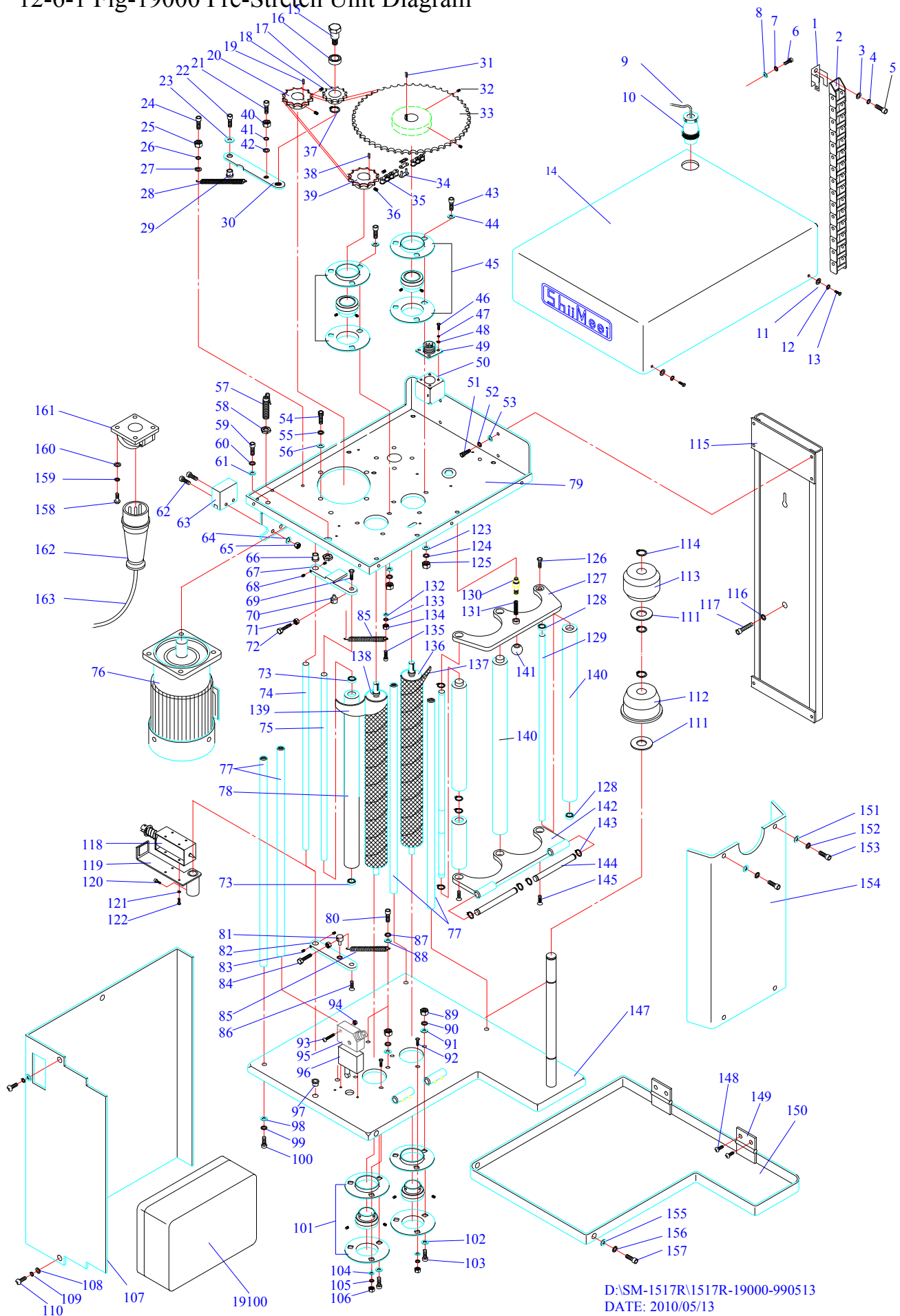
12-6-1 Fig-19000 Pre-Stretch Unit Diagram
