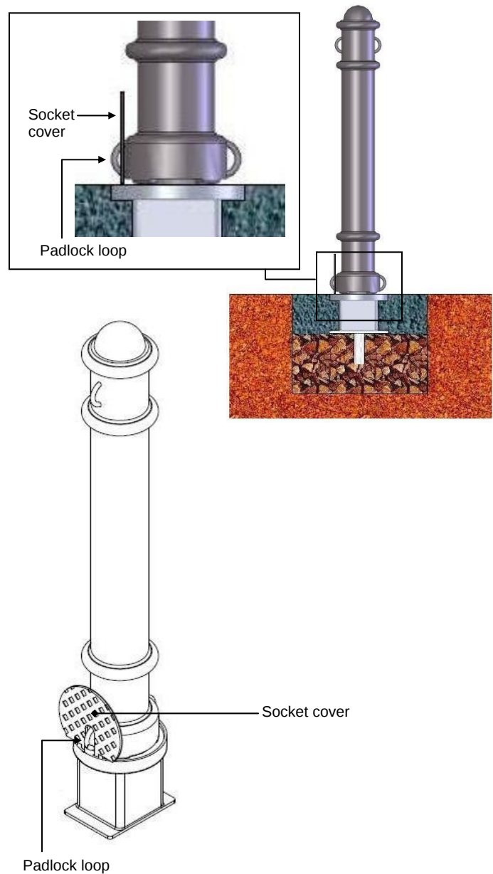
FIG. 5: Install bollard
