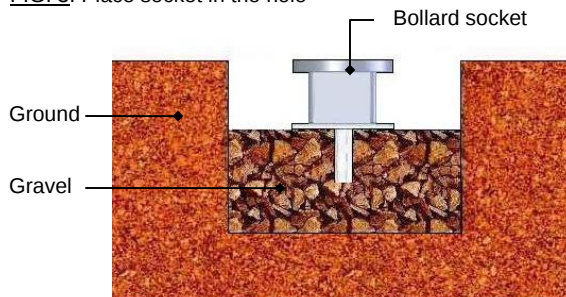
FIG. 3: Place socket in the hole
