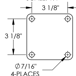
MOUNTING BRACKET SCALE: 1:4
