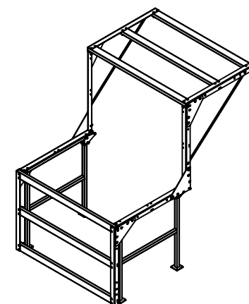
MOUNTING BRACKET SCALE: 1:4
