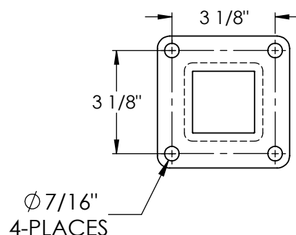
MOUNTING BRACKET DETAIL SCALE 1:4
