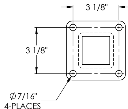
MOUNTING BRACKET DETAIL SCALE 1:4
