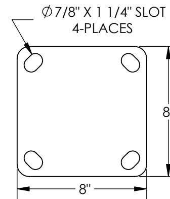
MOUNTING PLATE DETAIL, SCALE 1:6
