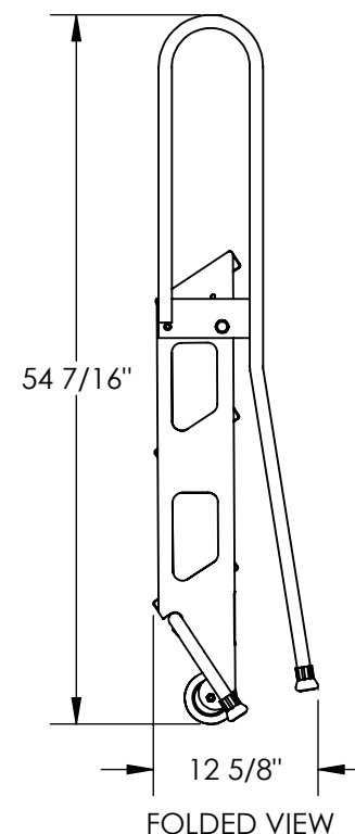
FOLDED VIEW
