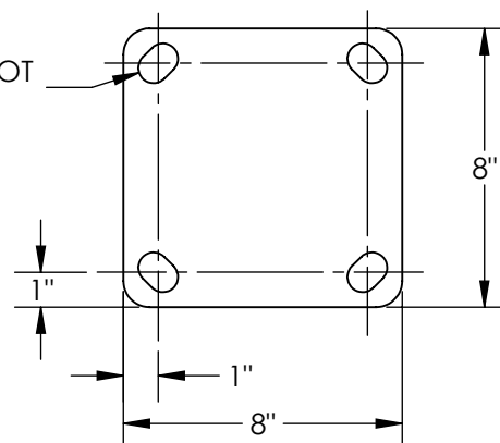
MOUNTING PLATE DETAIL, SCALE 1:6
