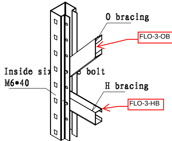
Upright & Bracings
