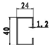
Bracing section
