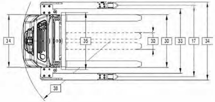
Mast table PSE 26NSL
