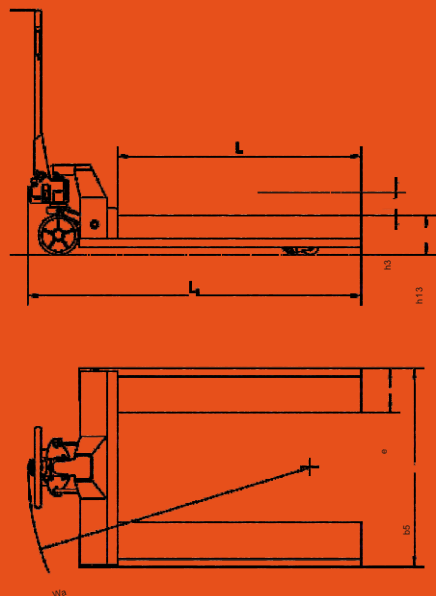
“Reel Carrying Truck” designed for carrying horizontal transport loads such as rolls, reels, cable drums etc.
