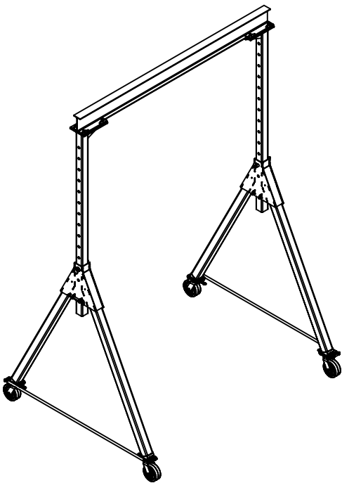
3D VIEW FOR REFERENCE ONLY DIMENSION TOLERANCE ± 1/4"
